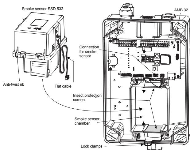
Fig. 3 Deploying the smoke sensors
